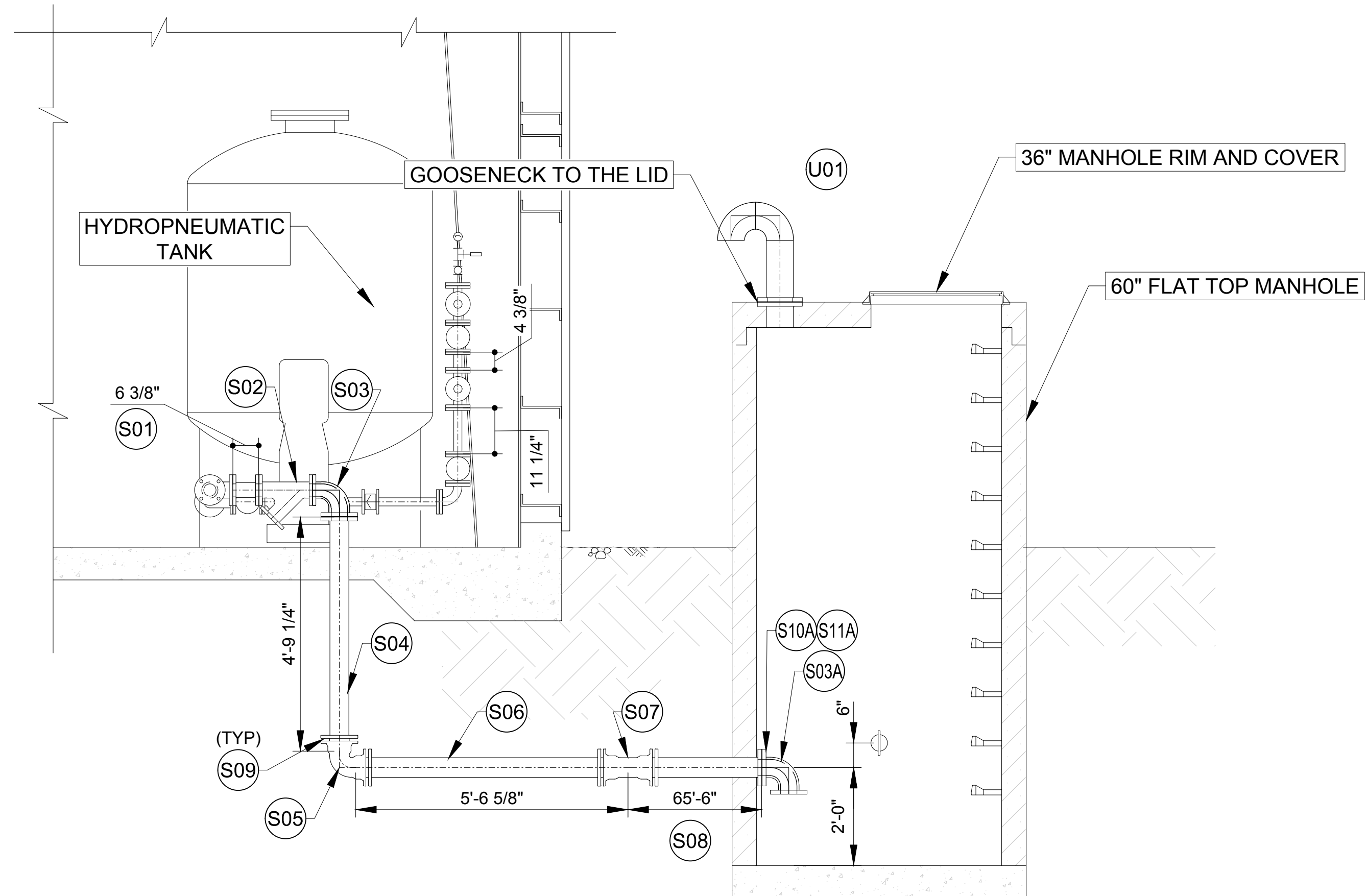
SECTION - B
