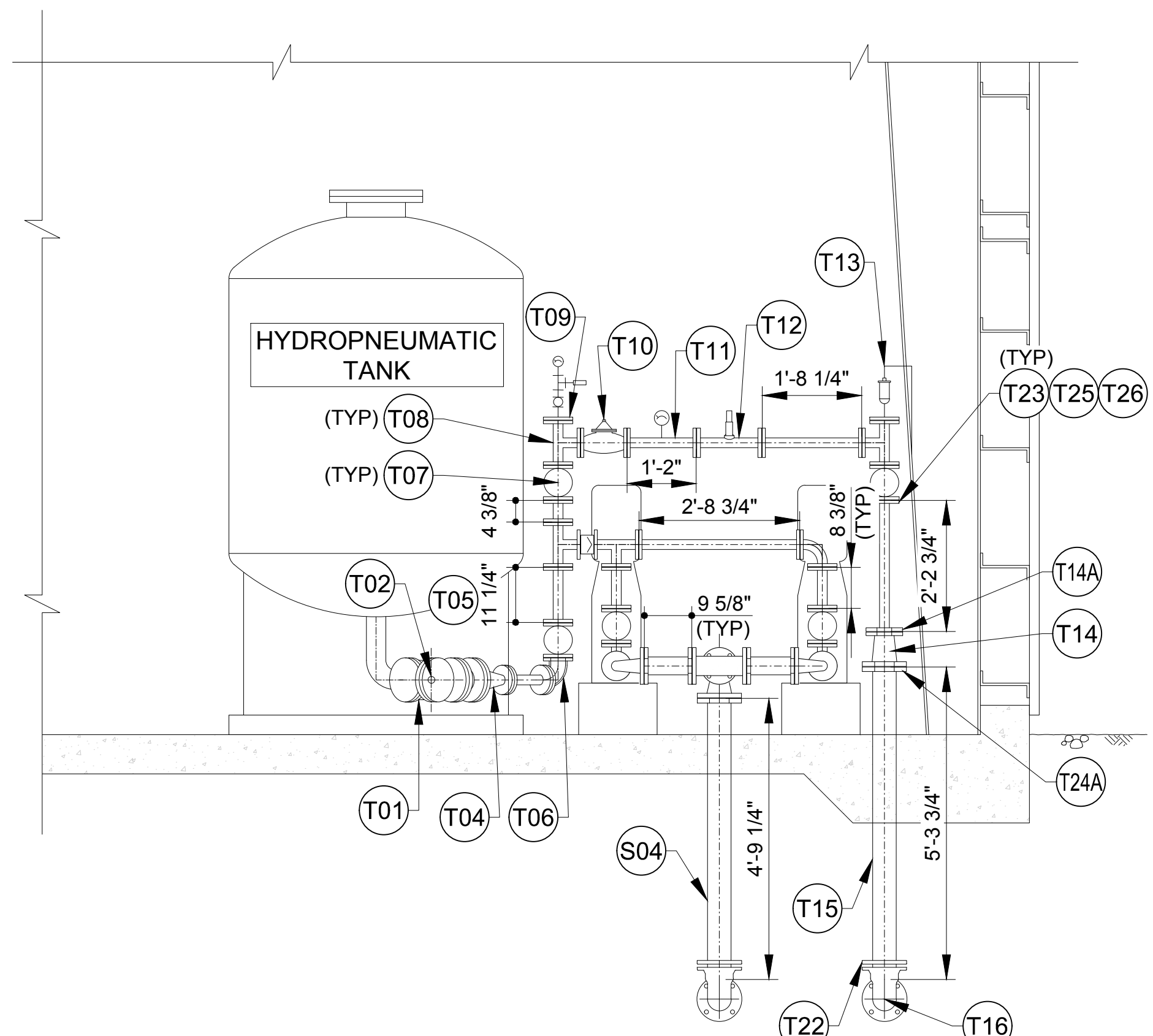
SECTION - A
